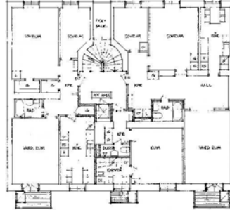
Plan 4
