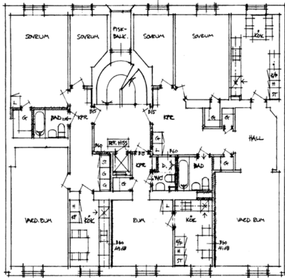
Plan 4-5
