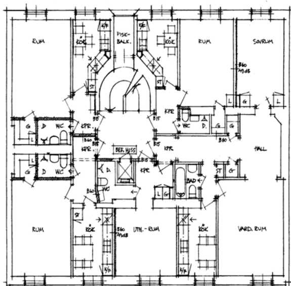
Plan 1-3
