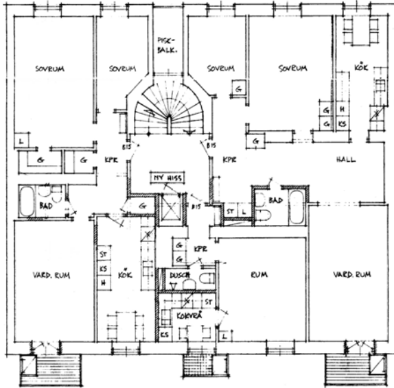
Plan 4
