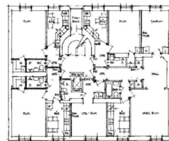
Plan 1-3
